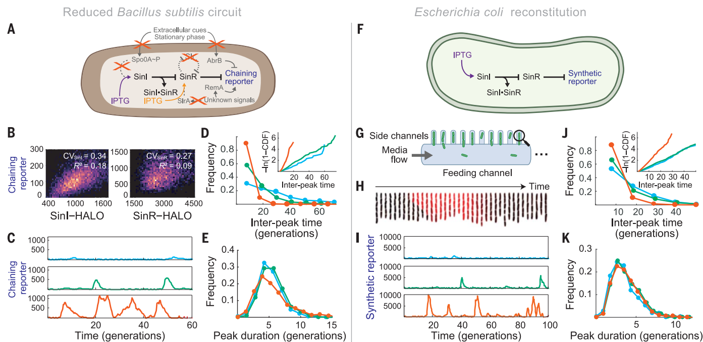
Fig. 2. Stochastic competition drives cell fate switching. (A) Genetic logic of the reduced B. subtilis circuit. System output was monitored by using a chaining reporter gene ( P_{\text{tapA}}\text{-}cfp ). (B) Single-cell SinI-HALO (TMN-1227, \Delta\text{sinI } \Delta\text{slrR } ynf/yloA::P_{\text{sinI}}\text{-sinI-HALO } P_{\text{tapA}}\text{-}cfp ) and SinR-HALO (TMN-1229, \Delta\text{sinR } \Delta\text{slrR } ywrK::P_{\text{sinR}}\text{-sinR-HALO } P_{\text{tapA}}\text{-}cfp ) expression distributions. (C) Example traces of chaining reporter expression in the reduced B. subtilis strain (TMN-1159, \Delta\text{sinI } \Delta\text{slrR } P_{\text{spank}}\text{-sinI } P_{\text{tapA}}\text{-}cfp P_{\text{hag-mKate2 } hag233V} ) grown in 7.5 \mu\text{M} (blue), 10 \mu\text{M} (green) and 12.5 \mu\text{M} (orange) IPTG. Measurements of P_{\text{spank}} promoter activity (fig. S2) suggest that growth in 7.5 \mu\text{M} , 10 \mu\text{M} and 12.5 \mu\text{M} IPTG lead to relative SinI expression levels of 0.4, 0.7, and 1.0, respectively. (D and E) Quantitative properties of the reduced B. subtilis system. Curve colors are matched with the data in (C). (D) Distribution of interpeak times. (Inset) Log-transformed cumulative distribution of interpeak times. (E) Distributions of chaining reporter peak durations.
