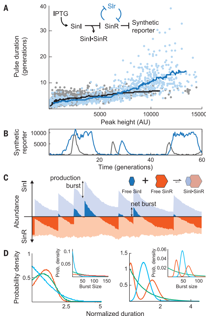
Fig. 3. Tuning commitment to the ON state.
