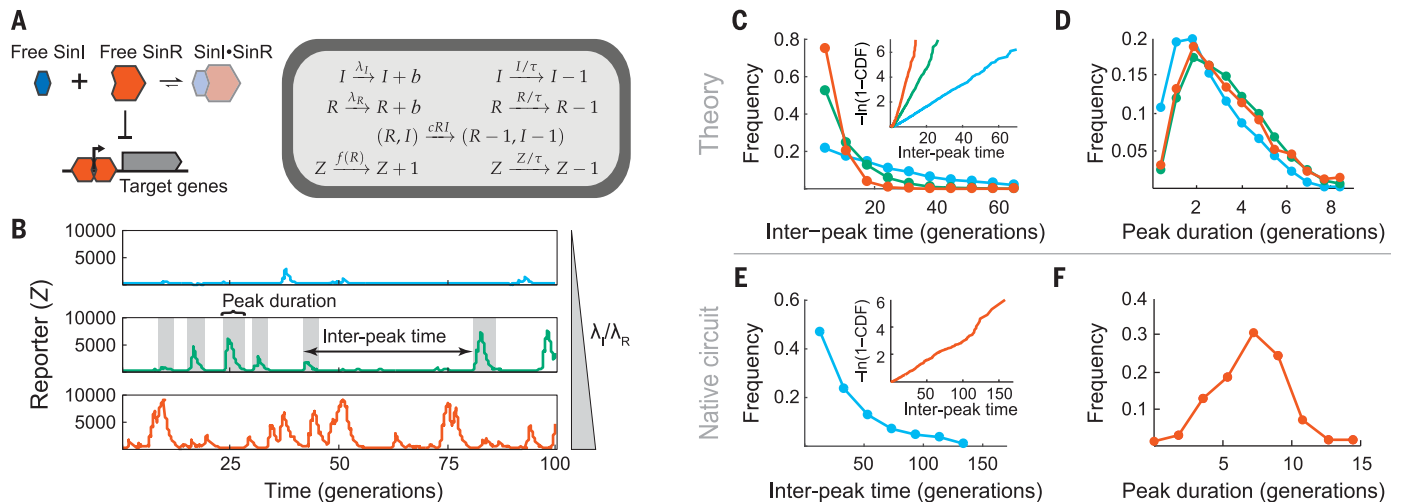
Fig. 1. A simple stochastic competition model can quantitatively explain switching. (A) (Left) Logic of the SinI-SinR regulatory motif. SinI neutralizes SinR by sequestering it away from target promoters and into an inert complex (shaded). When unbound by SinI, SinR represses the chaining regulon. (Right) A simple model implementing stochastic competition. SinI and SinR ( I and R ) are produced with constant probabilities \lambda_I and \lambda_R and form complexes with rate cRI . R represses the synthesis of a target, Z , and all components are presumed stable with average lifetime \tau . I and R are assumed to be produced one at a time for the simulations in this figure (i.e., b = 1 ). Formal treatment of the model can be found in the mathematical derivations section of the SM. (B) Realizations of stochastic competition. Component lifetimes were set to one generation to capture dilution due to cell growth, and complex formation was rapid relative to dilution. \lambda_I/\lambda_R
